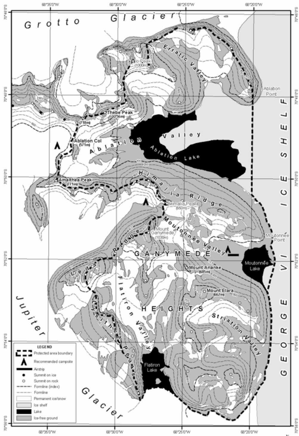
Map 2. Ablation Valley and Ganymede Heights ASPA No. 147, topographic map Alexander Island, Antarctic Peninsula
